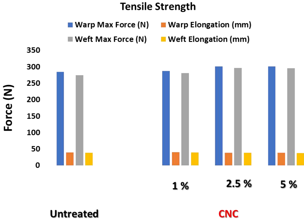
Figure 2: Strength of treated and untreated samples by CNC.
