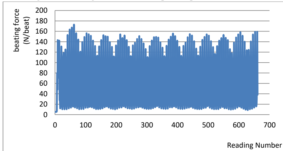
Fig (5) The beating force used at (280rpm),(15 picks/cm),(12/1 Ne).
