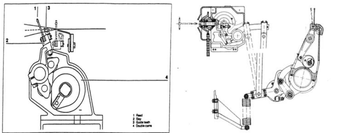
Fig (1) Beating mechanism of weaving m/c Fig(2)Double beat-up position of terry m/c
