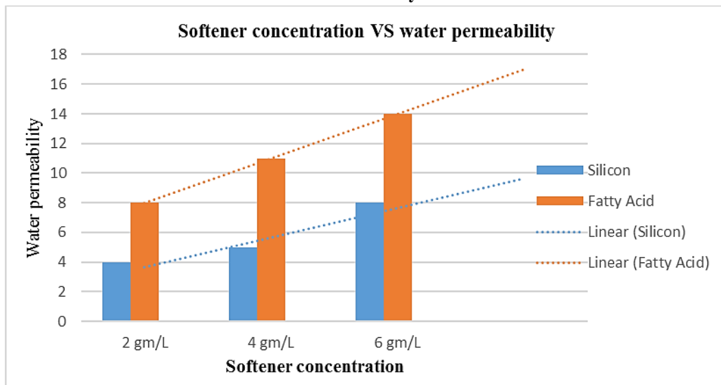
Figure-4: water permeability after applying different amount of silicon Softener and Fatty Acid.
