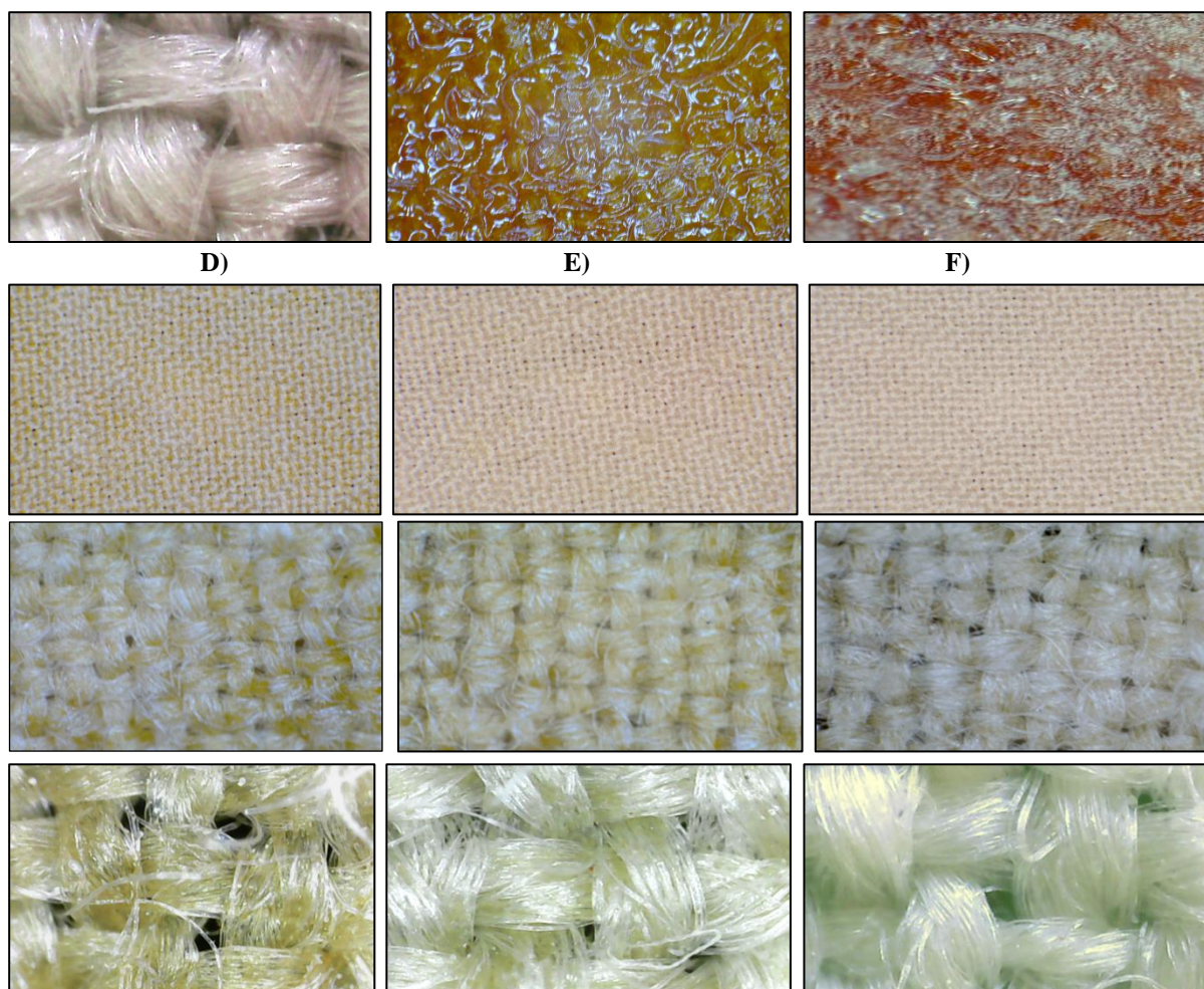
Figure (2): graphs and SM micro-graphs of the samples before and after PU removal, a. the pure wool, b. the PU-brushed samples, c. the PU-brushed samples after aging (APS), d. graph and 2 SM micro-graphs of APS-F1, e. graph and 2 SM micro-graphs of APS-F2, f., graph and 2 SM micrographs of APS-F3.
